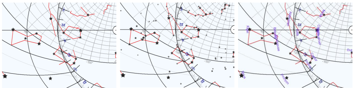
star up to magnitude 2
