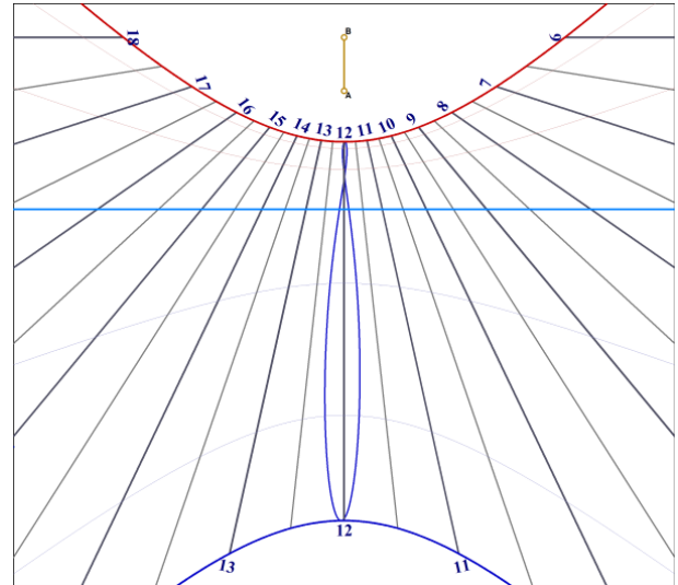
Vertical sundial for the city of Cape Town, South Africa, of latitude 33^{\circ} 55' south. The June solstice arc is at the top part (Winter), the December arc is at the bottom part (Summer). Hours go from the right (morning) to the left (afternoon). The sundial is due north.
