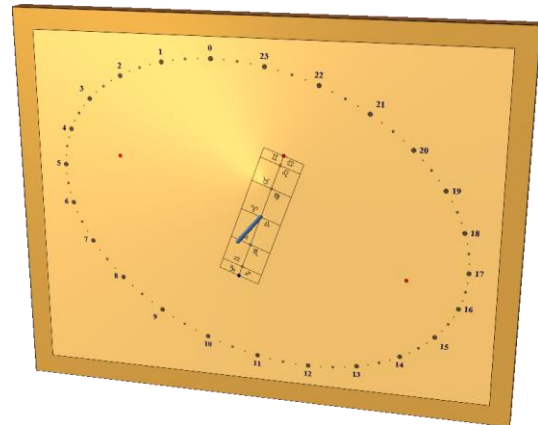
Vertical declining analemmatic sundial (20° east)
