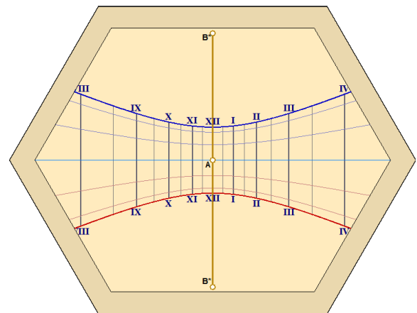
Hexagonal plate
