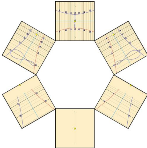
Left: An example of a multiple polar sundial on a hexagonal cylinder. Imagine that each sundial is folded on the sides of a cylinder. Declinations are 60^\circ , 120^\circ , and 180^\circ around the polar axis.
