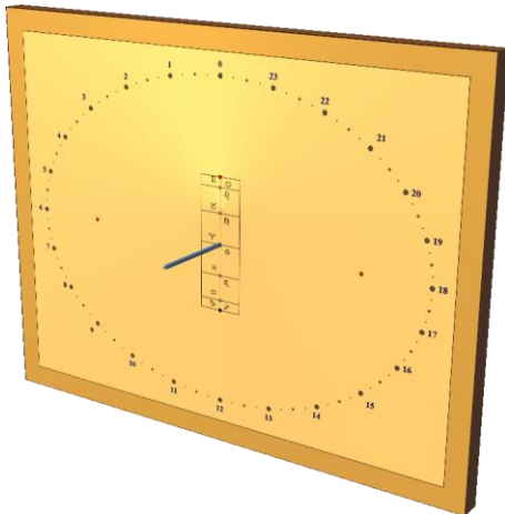
Vertical direct south analemmatic sundial
